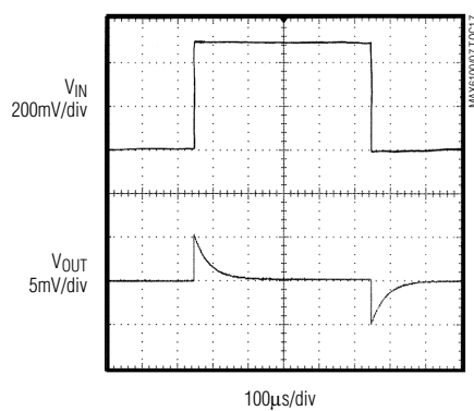
MAX6105 LINE-TRANSIENT RESPONSE
