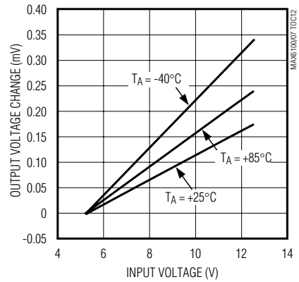
MAX6105 LINE REGULATION
