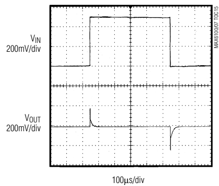
MAX6101 LINE-TRANSIENT RESPONSE
