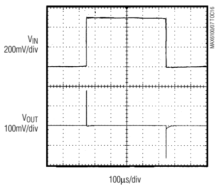
MAX6102 LINE-TRANSIENT RESPONSE
